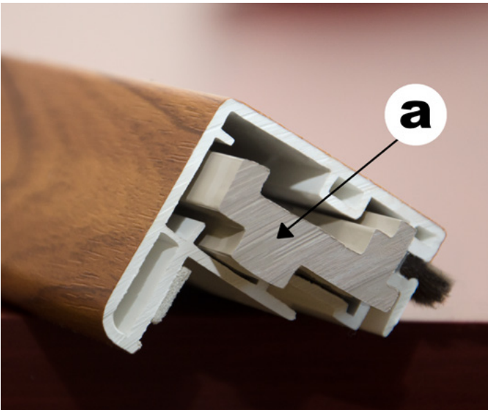
Additional high density composite reinforcement (a) inside the locking sash makes our windows structurally stronger than others available on the market.
